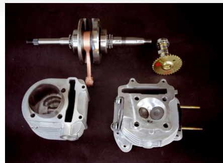
GY6 oversize cylinder Kit 2V ( 232.69cc )
